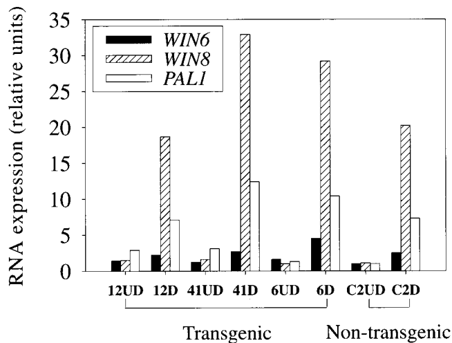
Fig. 4. Expression of several defense-related genes before and after induction via mechanical wounding of leaves. RNA samples were collected from leaves of undamaged (UD) and damaged (D) trees. Data are from two moderate b0-expressing lines (12 and 41), the high b0-expressing line 6, and the non-transgenic line (C2) from clone 195-529. The levels of gene expression were quantified from Northern analysis after standardization based on rDNA expression. No significant differences in expression level for PALL and WIN genes were detected in any of the transgenic lines when compared with its control, C2.
